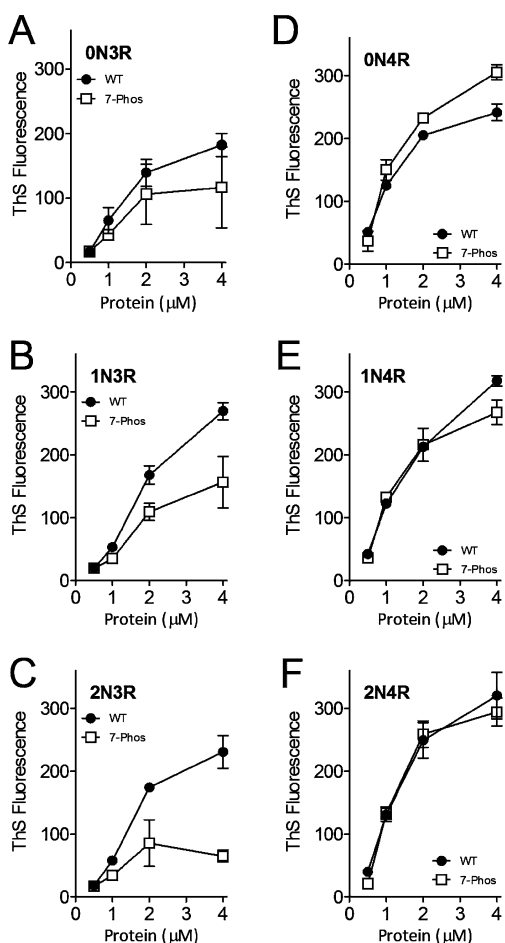
Figure 2. Polymerization of varied tau concentrations measured by thioflavin S staining. Wild-type (●) and 7-Phos tau isoforms (□) polymerization reactions with 0–4 \mu\text{M} protein (x-axis) and 75 \mu\text{M} arachidonic acid were measured by thioflavin S fluorescence (y-axis) after 18 h incubation at 25 ^{\circ}\text{C} . Individual graphs are shown for (A) 0N3R, (B) 1N3R, (C) 2N3R, (D) 0N4R, (E) 1N4R, and (F) 2N4R isoforms. Bars represent the mean from 3 experiments \pm SD.
