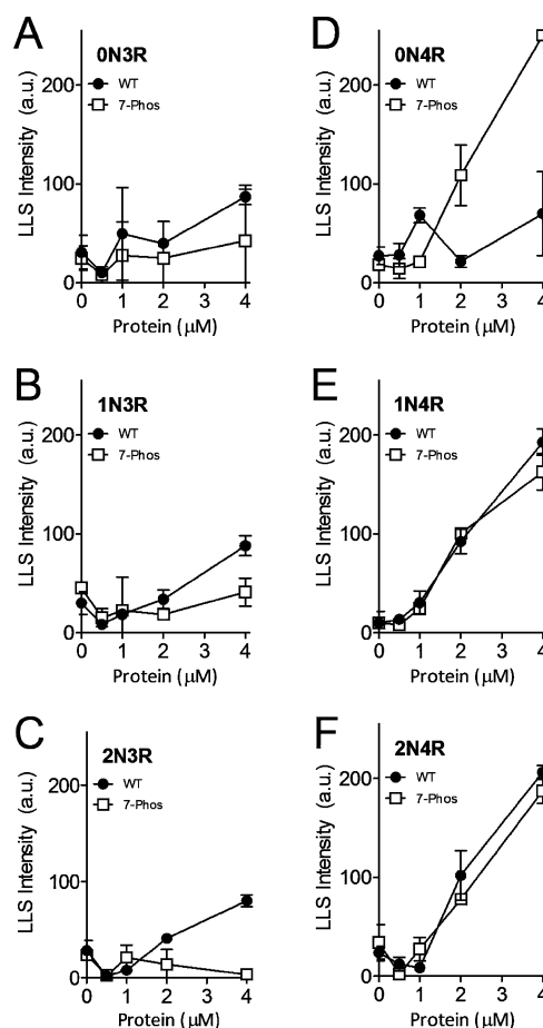
Figure 3. Polymerization of varied tau concentrations measured by right-angle laser light scattering. Wild-type (●) and 7-Phos tau isoform (□) polymerization reactions with 0–4 \mu\text{M} protein (x-axis) and 75 \mu\text{M} arachidonic acid were measured by intensity of right-angle laser light scattering (y-axis) after 18 h incubation at 25 ^{\circ}\text{C} . Individual graphs are shown for (A) 0N3R, (B) 1N3R, (C) 2N3R, (D) 0N4R, (E) 1N4R, and (F) 2N4R isoforms. Data are the mean from 3 experiments, and bars represent \pm SD.
