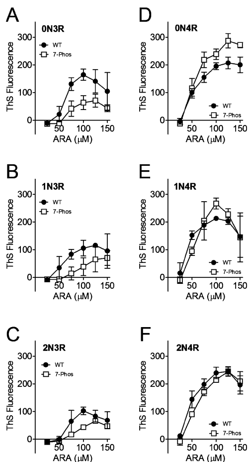
Figure 4. Polymerization of 2 \mu\text{M} tau with 0–150 \mu\text{M} ARA measured by thioflavin S fluorescence. Wild-type (●) and 7-Phos tau isoform (□) polymerization reactions with 2 \mu\text{M} protein, and 0–150 \mu\text{M} arachidonic acid (x-axis) was measured by thioflavin S fluorescence (y-axis) after 18 h incubation at 25 °C. The fluorescence value of the 0 \mu\text{M} ARA reaction was subtracted from the other values. Individual graphs are shown for (A) 0N3R, (B) 1N3R, (C) 2N3R, (D) 0N4R, (E) 1N4R, and (F) 2N4R isoforms. Bars represent \pm\text{SD} from 3 experiments.
